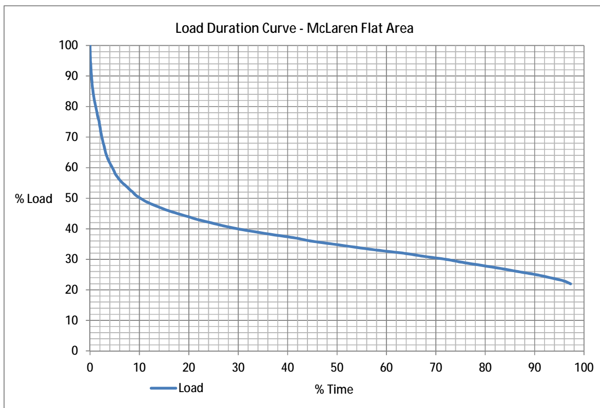
Figure 3 Load duration curve - McLaren Flat area
