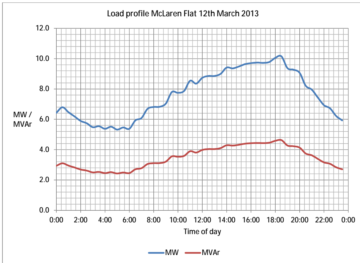
Figure 2 Load profile McLaren Flat
