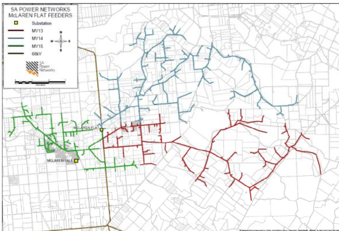
Figure 1 Locality of McLaren Flat Substation
